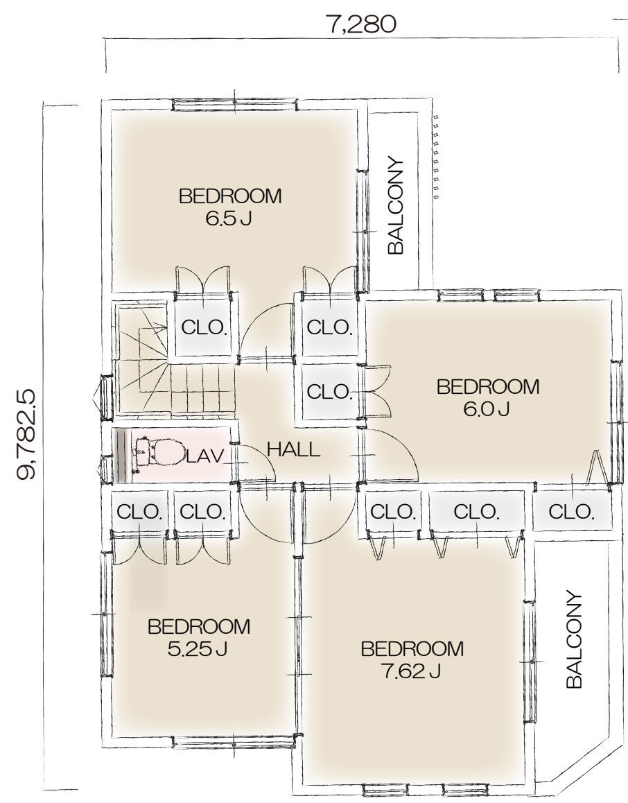
2F PLAN
