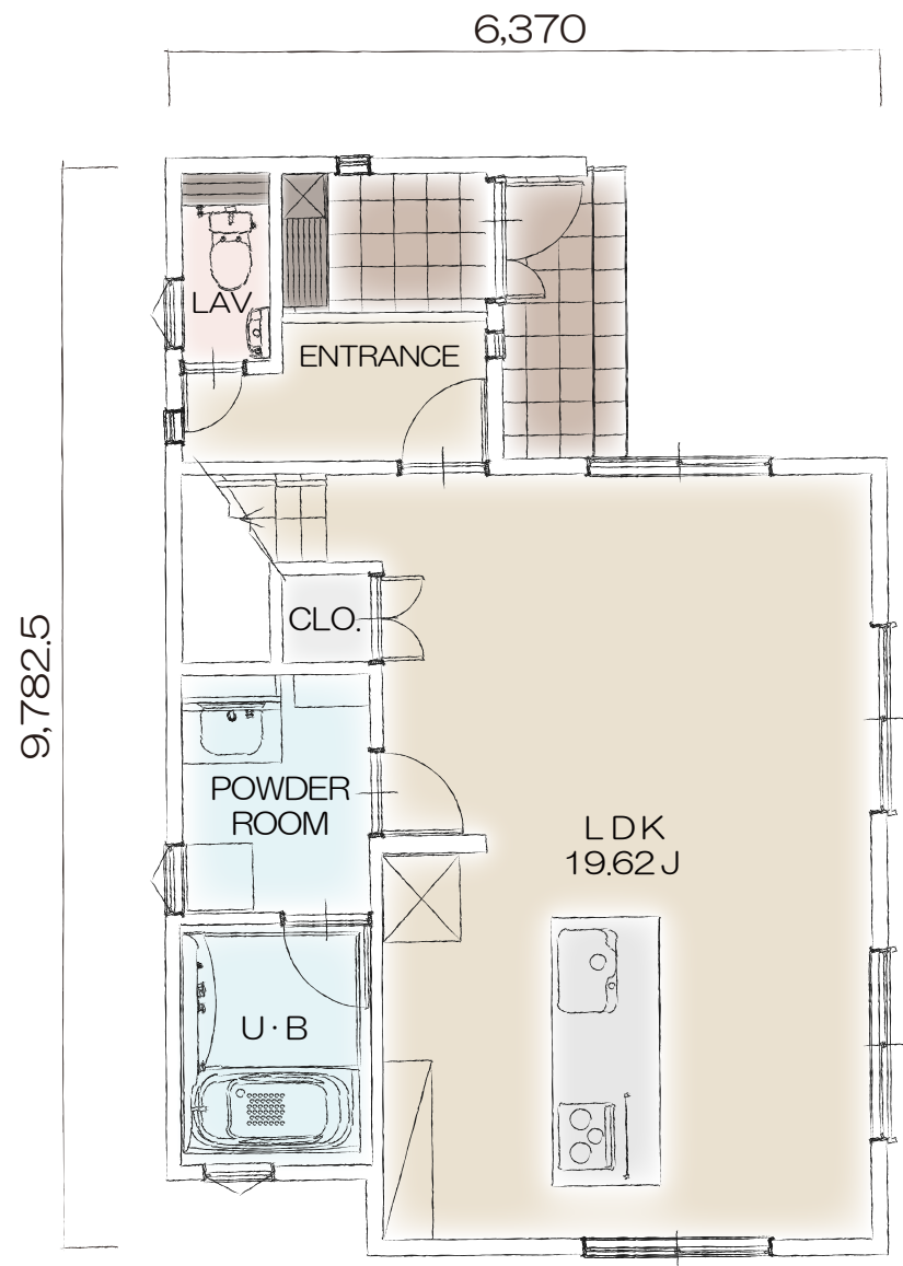
1F PLAN
